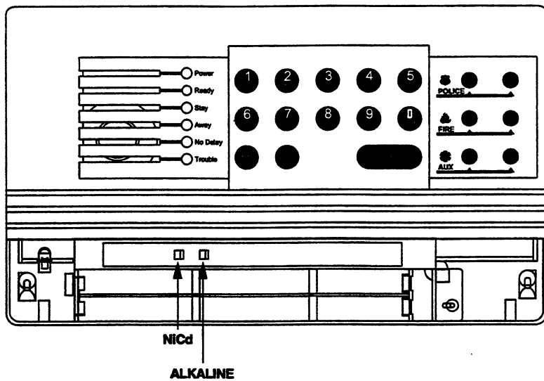
Figure 6. Tab Indicates Battery Type Installed
